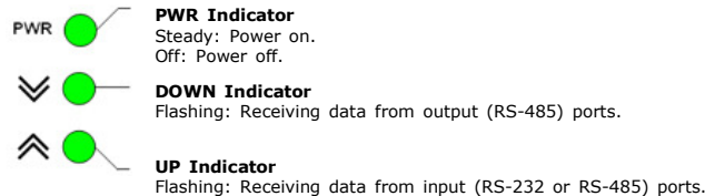
FIGURE 2: LED INDICATIONS
