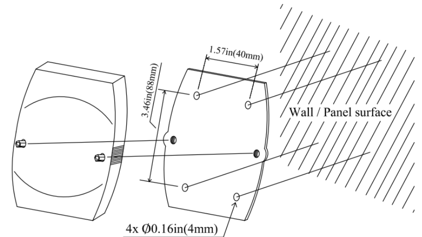
FIGURE 4: WALL/PANEL MOUNTING
